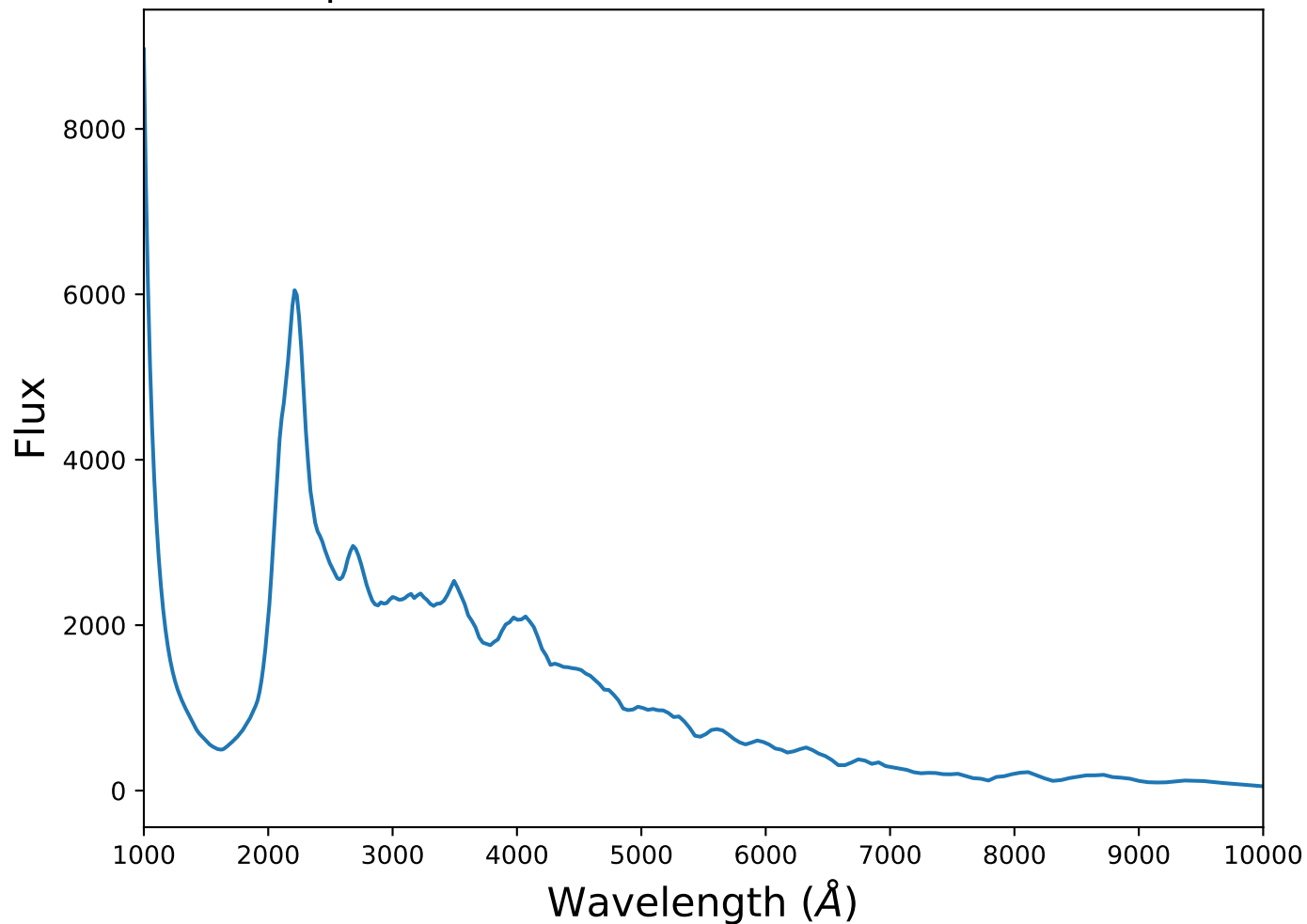
Spectrum 6 for transient SNIa at z=0.59
